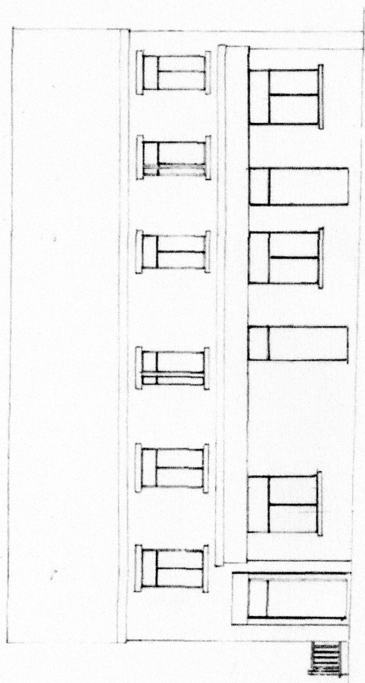
Prop Front Elev
